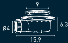
Válvula incluida / Valve included
